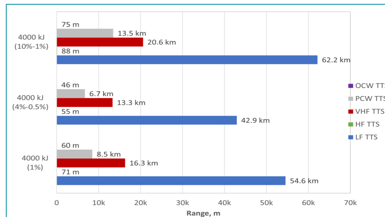
Figure 4.4: Modelled TTS Injury Ranges for Marine Mammals for Installation of Two Piles Concurrently, Using Energy Conversion Factors of 1%, 4% Reducing to 0.5% and 10% Reducing to 1%
